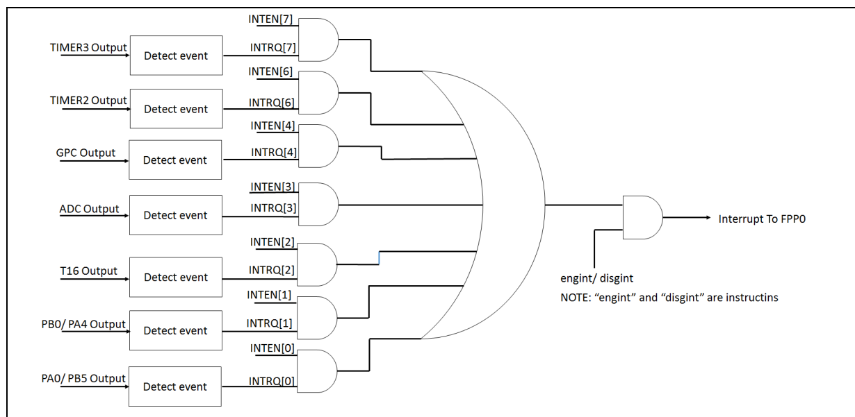
Fig. 16: Hardware diagram of interrupt controller
