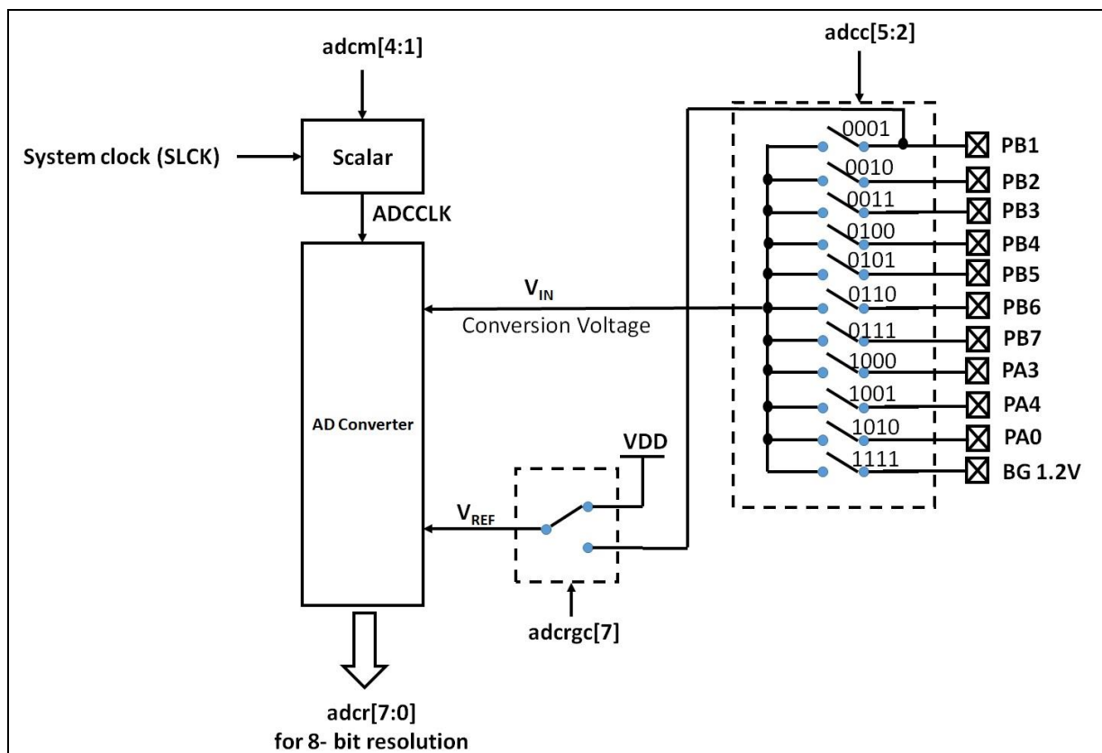
Fig. 19: ADC Block Diagram
