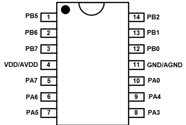
PMS171B-S14: SOP14 (150mil)
