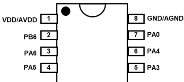
PMS171B-S08B: SOP8 (150mil)
