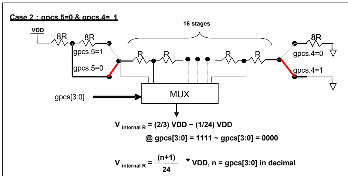
Fig. 6: V internal R hardware connection if gpcs.5=0 and gpcs.4=1
