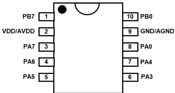
PMS171B-M10: MSOP10 (118mil)
