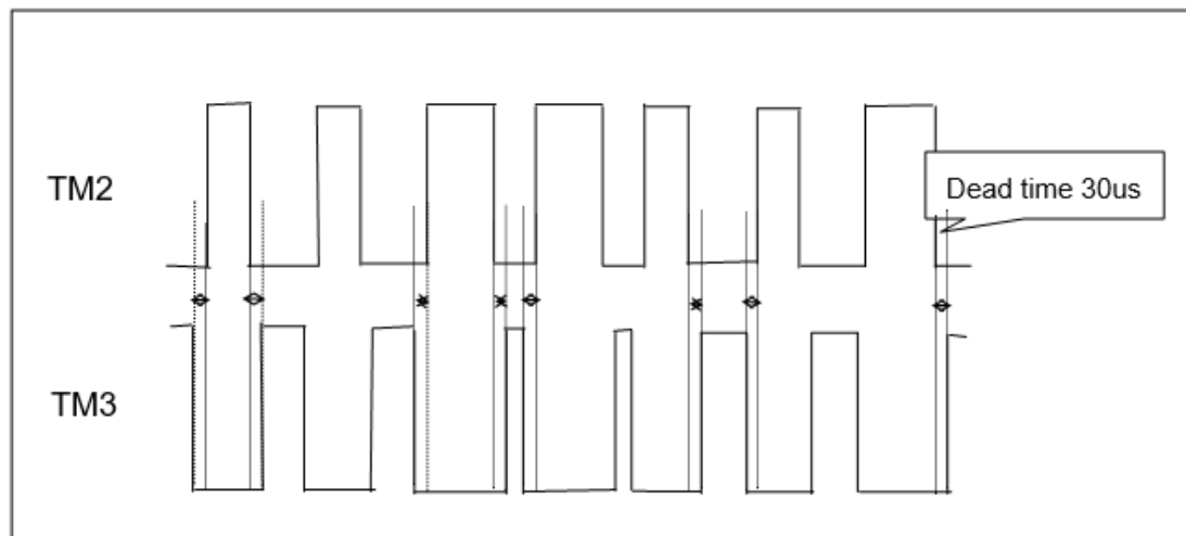
Fig. 14 : Two complementary PWM waveforms with dead zones
