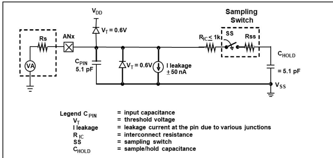
Fig.20: Analog Input Model
