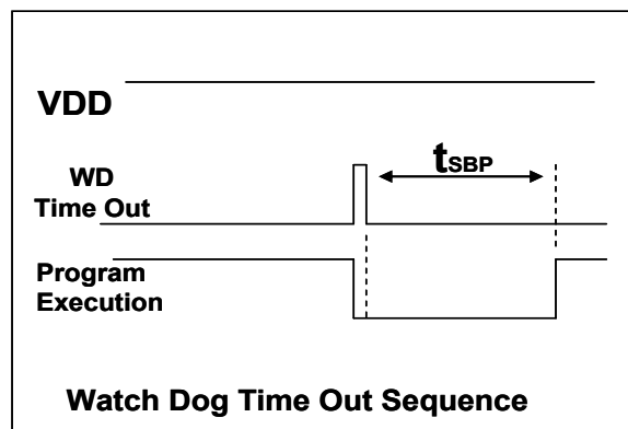
Fig. 15: Sequence of Watch Dog Time Out
