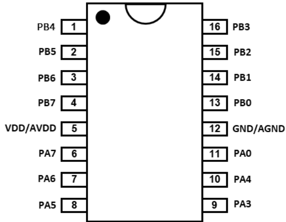
PMS171B-S16: SOP16 (150mil)
