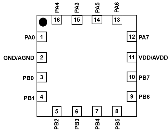
PMS171B-1J16A: QFN3*3-16pin (0.5pitch)
