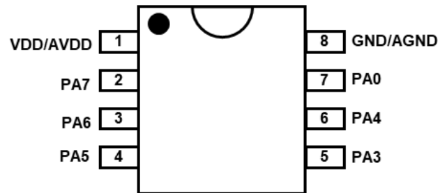
PMS171B-S08: SOP8 (150mil)
