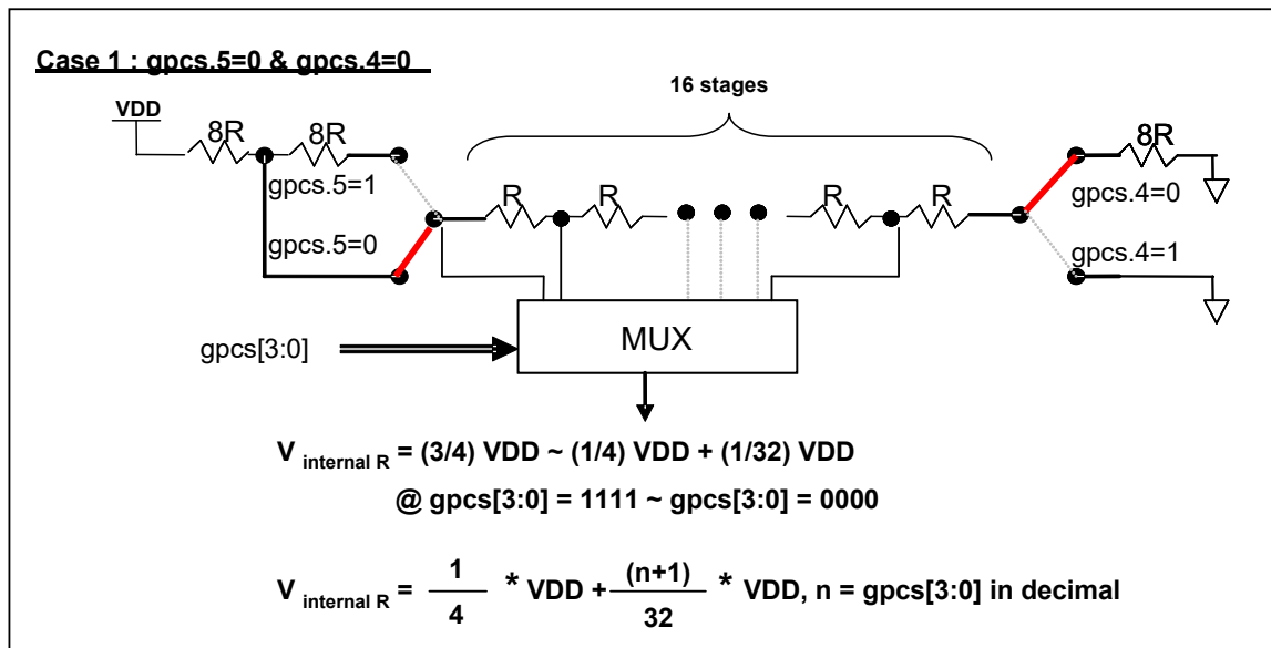
Fig. 5: V internal R hardware connection if gpcs.5=0 and gpcs.4=0
